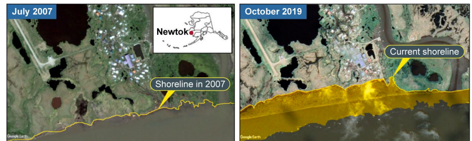
Shoreline Erosion at Newtok, Alaska, from July 2007 to October 2019.
